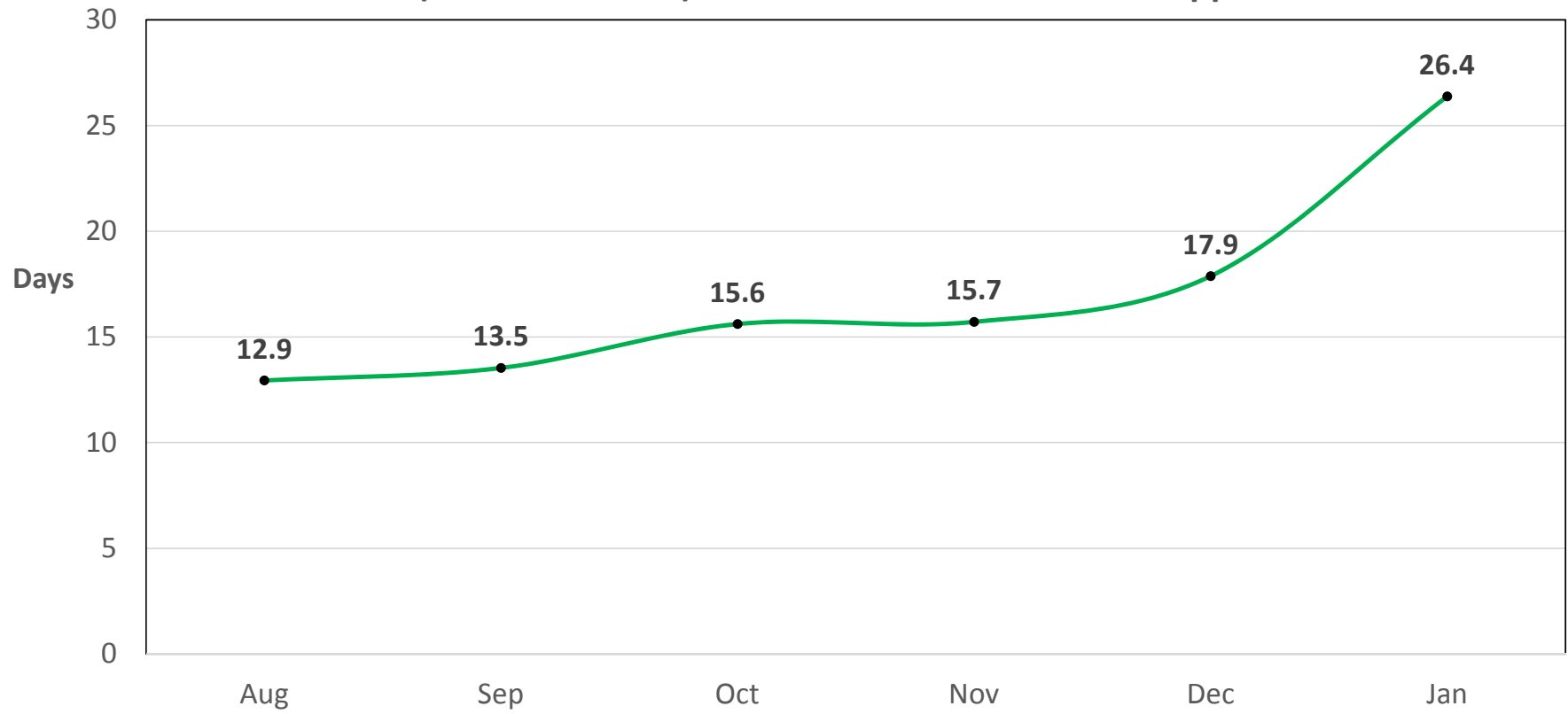
Average Trip Times - CP Originated Traffic to Vancouver Non Bulk Terminals (SRY Terminated) 2018-19 Grain Year for ATC Shippers
